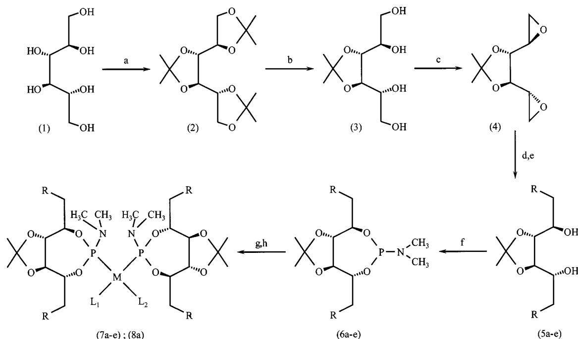
Figure 1. a) acetone, H 2 SO 4 ; b) AcOH, H 2 O, 40 °C; c) (i) trimethyl orthoacetate, PPTS, (ii) NEt 3 , AcBr, (iii) K 2 CO 3 , MeOH; d) LiAlH 4 , Et 2 O, R = H; e) CuBr·SMe 2 , RMgBr, THF/Et 2 O, -40 °C, R = CH 3 , C 2 H 5 , i-C 4 H 9 , C 6 H 5 ; f) HMTAP, toluene, reflux; g) Rh I (COD) 2 -(SO 3 CF 3 ), CH 2 Cl 2 , 7a-e ; M = Rh, L 1 -L 2 = COD; h) Pd II (COD)Cl 2 , CH 2 Cl 2 , 8a ; M = Pd; L 1 , L 2 = Cl
