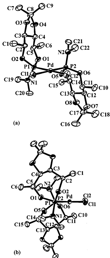
Figure 2. Molecular structure of 8a ; (a) front view: square-planar environment of Pd II ; (b) side view: C 2 -symmetric arrangement; hydrogen atoms have been omitted for clarity
